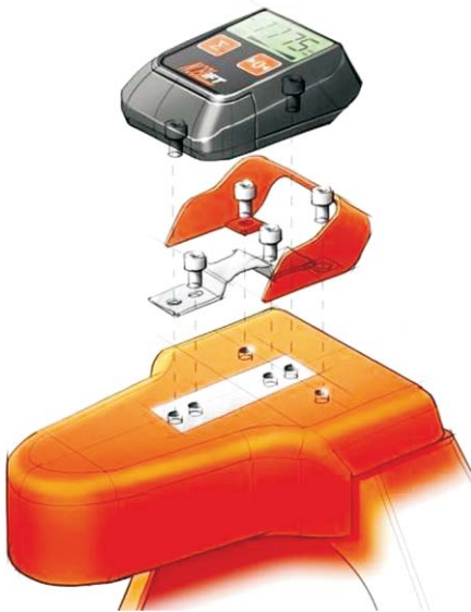
Schematic exploded view of product configuration
